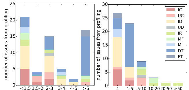
(a) Server-time speedup (x) (b) Line of code changes Figure 10: Performance fixes and LOC involved
