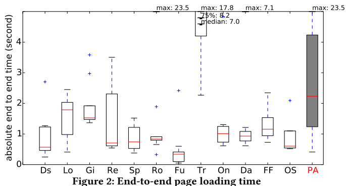
Figure 2: End-to-end page loading time Measured for top 10 time-consuming pages per application. Box: 25 to 75 percentile; Red line: median; PA: problematic actions from all 12 applications (see Section 3.2).
