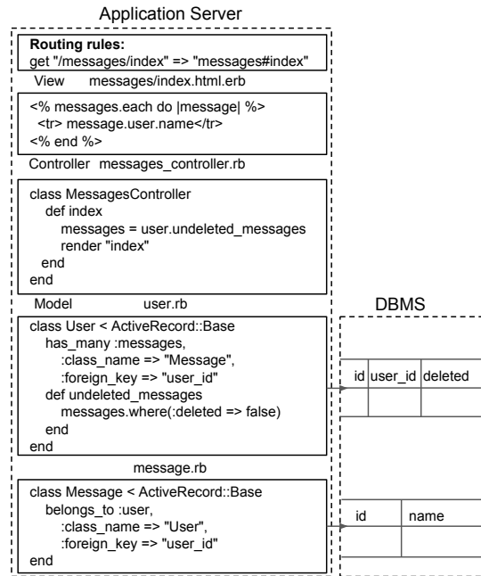
Figure 1: Structure of an example Rails application
